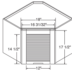
AC2417.5 DIAGONAL
