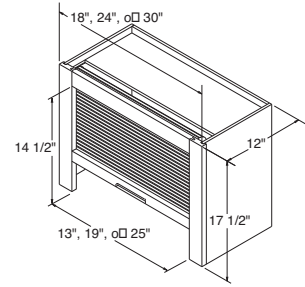
ACS1817.5-ACS3017.5 STRAIGHT
